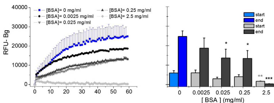
Fig. 7. Effect of albumin protein concentration (0–2.5 mg/ml). Left: Adsorption kinetics was measured for 60 min, the ctrl condition is indicated in blue. Right: Startpoints (light gray bars) and endpoints (dark gray bars) are shown. Albumin concentration inhibited LBPs adsorption rate in a dose-dependent manner.
