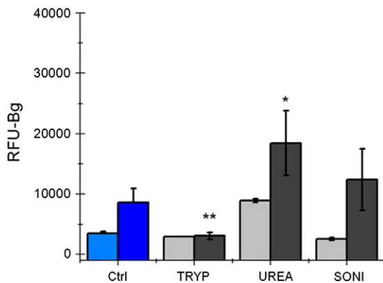
Fig. 8. Stability of LBPs. Adsorption of LBPs pretreated with 1% trypsin, 1 M urea and sonification (70 peak/W) respectively. Proteolysis of LBPs significantly decreases their adsorptive capacity.
