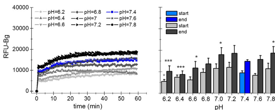
Fig. 3. Effect of pH (pH 6.2–7.8) on LBPs. Left: Adsorption kinetics was measured for 60 min, the ctrl condition is indicated in blue. Right: Startpoints (light gray bars) and endpoints (dark gray bars) are shown. Maximal adsorption was occurred at pH 7.0 and 7.8, acidic conditions (pH 6.2 and 6.4) significantly reduced LBPs adsorption.
